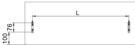
Pre-drilling guide
